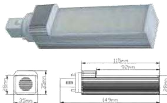
G24-SMD44S
